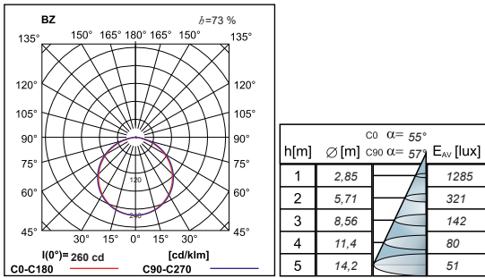
ARTSHAPE ROUND LED MEDIUM FULL 8000LM PLX 840 Z-1,5M
